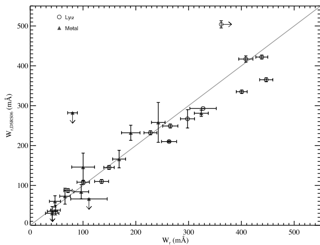
FIG. 20.—Comparison of rest equivalent widths from our analysis with D06. The D06 values are plotted over the values measured in the current paper, and the one-to-one relation is shown (solid line). The circles are for Ly \alpha W_r , and the triangles are for metal lines (i.e., C III and O VI). D06 use COG concordance plots, Voigt profile fits, and/or the AODM to measure \log N_{\text{D06}} and b_{\text{D06}} , typically assuming a single component. From \log N_{\text{D06}} and b_{\text{D06}} , they measure W_{r,\text{D06}} . They tend to underestimate W_{r,\text{D06}} compared to our values, which are a simple sum of the absorbed flux and include unresolved components. [See the electronic edition of the Journal for a color version of this figure.]
