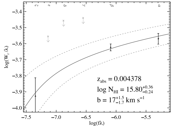
FIG. 2.—H I COG for z_{\text{abs}} = 0.00438 . The best-fit curve of growth (solid line) with 1 \sigma bounds (dashed lines) is displayed over the measured W_r values included in the fit (black marks with 1 \sigma error bars). Blended lines are shown as upper limits (crosses and arrows). For description of the upper limits, see Fig. 1. The H I Lyman lines are labeled by letter or wavelength across the top. [See the electronic edition of the Journal for a color version of this figure.]
