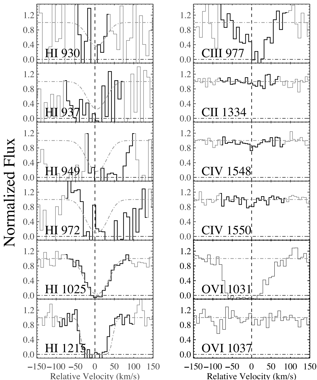
FIG. 1.—Velocity plot for z_{\text{abs}} = 0.00438 . Spectra, averaged over 2 pixels (thin black line), are stacked in velocity space with v = 0 \text{ km s}^{-1} at z_{\text{abs}} = 0.00438 , the optical depth weighted centroid of \text{Ly}\alpha (vertical dashed line). The region used to measure W_r is highlighted (thick black line). Also indicated is the flux at zero (black dot-dashed line). The H I Voigt profiles, based on the COG \log N_{\text{H I}} and b , are superimposed to show the predicted area under the curve (gray dot-dashed line; for the metal lines, this line indicates the flux at unity). The Voigt profile centroid is fixed at the redshift of \text{Ly}\beta , z_\beta = 0.00439 . \text{Ly}\alpha is detected in the wings of the damped Galactic \text{Ly}\alpha feature, and the lines higher than \text{Ly}\beta are detected in the SiC 2A and 1B channels, which have poor sensitivity. C II and C IV \lambda 1550 are not detected at 3 \sigma . \text{Ly}\gamma , \text{Ly}\delta , and \text{Ly}\epsilon are blended with Galactic C III, \text{H}_2 \lambda 954.0 R(4) , and \text{H}_2 \lambda 941.6 P(2) , respectively. As shown, Galactic C II \lambda 1036 is coincident where O VI \lambda 1031 would be, and there is an absence of O VI \lambda 1037 . [See the electronic edition of the Journal for a color version of this figure.]
