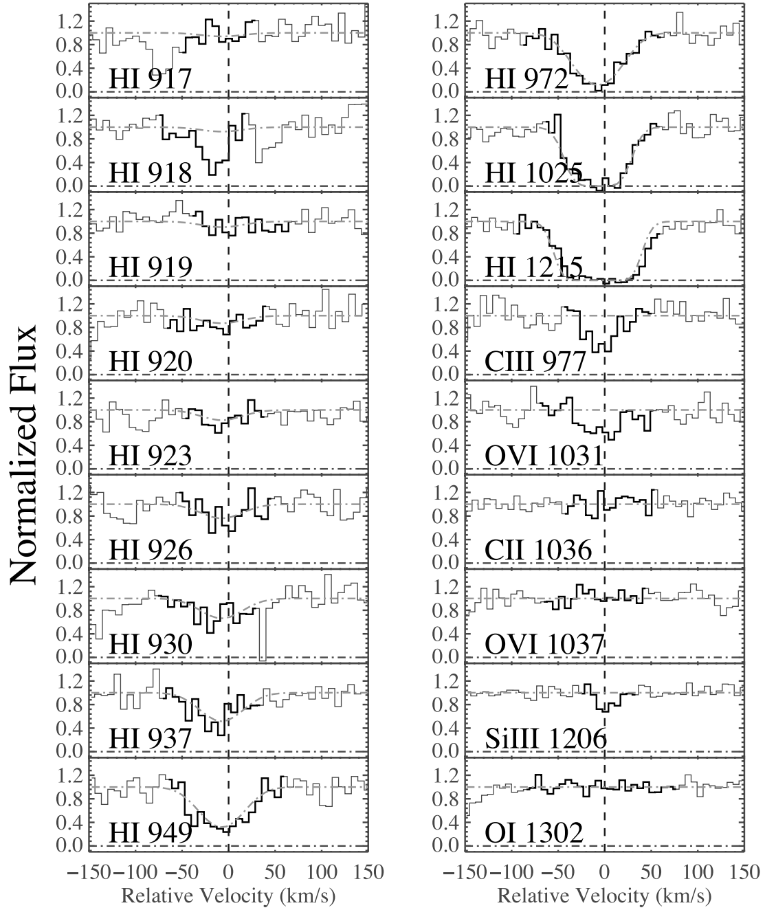
FIG. 16.—Velocity plot for z_{\text{abs}} = 0.19161 (see Fig. 1 description). H I \lambda 917 , both C II lines, O I, Si III, and O VI \lambda 1037 are not detected at 3\sigma . H I \lambda 918 is blended with H 2 \lambda 1094.0 P(1). The Voigt profile centroid is fixed at z_0 = 0.19158 . [See the electronic edition of the Journal for a color version of this figure.]
