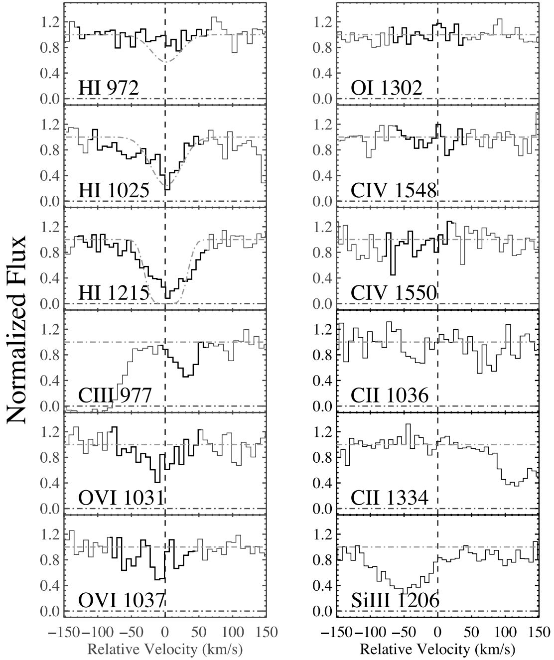
FIG. 5.—Velocity plot for z_{\text{abs}} = 0.06471 (see Fig. 1 description). \text{Ly}\alpha has a distinct asymmetric profile, probably due to unresolved components. The \text{O VI} doublet is detected at \approx 4.5\sigma . The W_r ratio of \text{O VI } \lambda 1031 to \lambda 1037 is 1.1 \pm 0.4 . \text{Ly}\gamma , \text{OI} , and \text{C IV} are not detected at 3\sigma . \text{C III} is treated as an upper limit since it is coincident with \text{H}_2 \lambda 1040.4 P(2) . The Voigt profile centroid is fixed at z_\beta = 0.06472 . [See the electronic edition of the Journal for a color version of this figure.]
