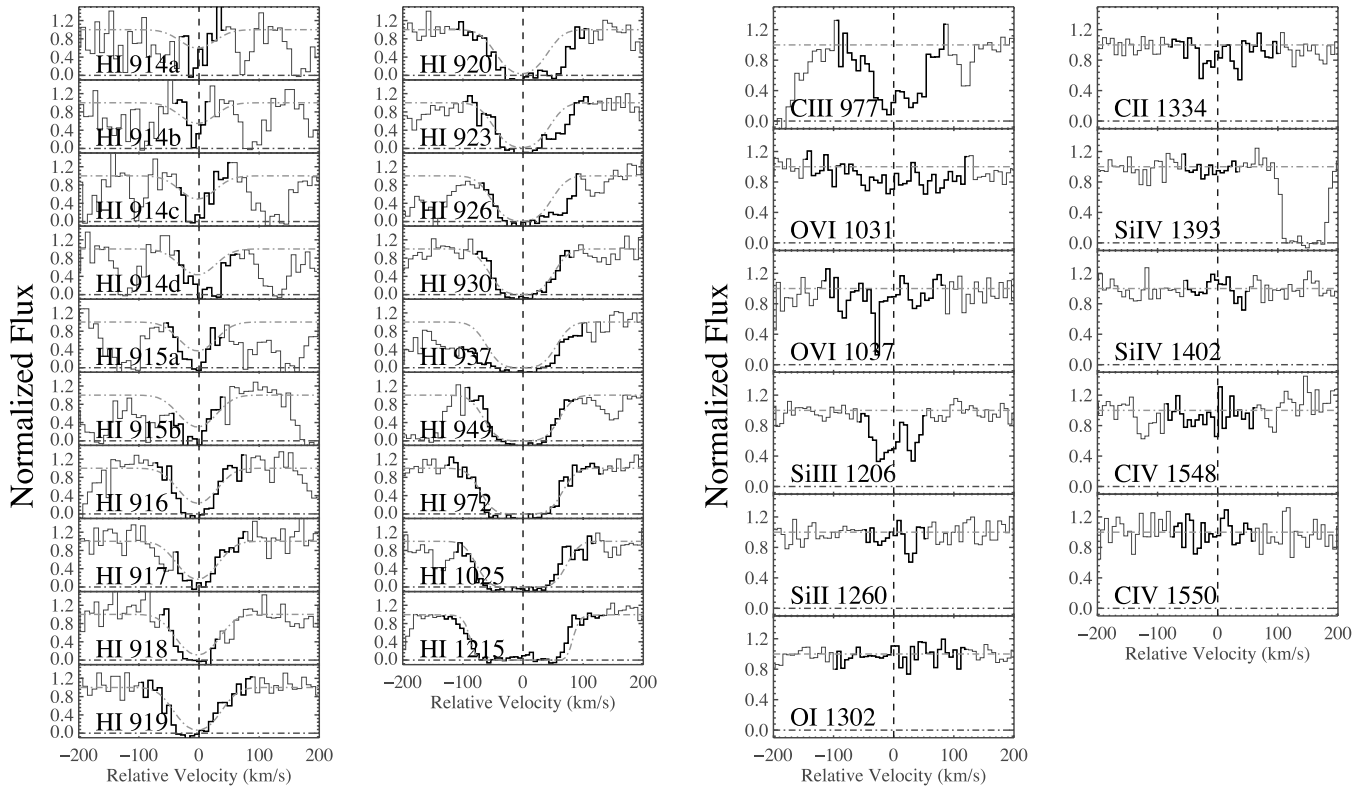
FIG. 9.—Velocity plot for the partial LLS at z_{\text{abs}} = 0.09487 (see Fig. 1 description). Ly \epsilon lies in the wings of the damped Galactic Ly \beta , and the higher order Lyman lines H I \lambda\lambda 914d, 916, 920, 923 , and 926 are blended or coincident with H _2 . For H I \lambda\lambda 917 and 918 , the H _2 blends, \lambda 1004.0 R(2) and \lambda 1005.4 P(2) , respectively, are excluded from the W_r measure. This system was used to shift the FUSE channels onto the STIS wavelength solution. The Voigt profile centroid is fixed at z_{915a} = 0.09486 . Ly \alpha , C III, C II, and Si III are well aligned, and they have similar, multicomponent profiles. A broad O VI doublet is detected at >3 \sigma . The W_r ratio of O VI \lambda 1031 to \lambda 1037 is 2.3 \pm 0.8 , in agreement with the predicted value for the unsaturated regime. Si II, O I, and the Si IV and C IV doublets are not detected at 3 \sigma . (Note: the horizontal limits are from -200 to +200 km s ^{-1} .) [See the electronic edition of the Journal for a color version of this figure.]
