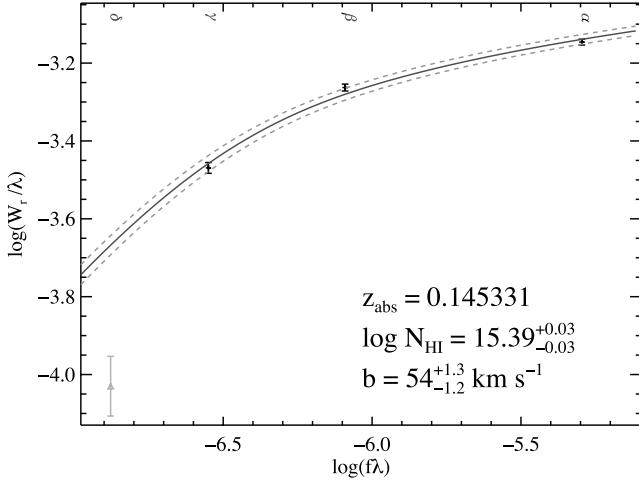
FIG. 15.—H I COG for z_{\text{abs}} = 0.14533 (see Fig. 2 description). The difference between the predicted and measured W_r of Ly \delta is significant and suggests that H I is multicomponent and poorly fitted by this single-component COG. [See the electronic edition of the Journal for a color version of this figure.]
