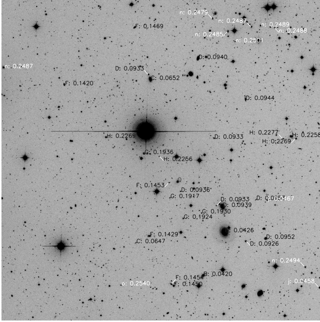
FIG. 23.—Galaxies with |\delta v_{\text{gal}}| \leq 1000 \text{ km s}^{-1} from metal-line systems and strong \text{Ly}\alpha absorbers. The former have capital letters indicating the system they neighbor, while the latter have lowercase letters. The systems at z_{\text{abs}} = 0.09400 and 0.09487 have most all neighboring galaxies in common; they are not labeled twice. Similarly for the systems at z_{\text{abs}} = 0.22555 and 0.22752 . The \text{O VI} systems are at z_{\text{abs}} = 0.04222, 0.06471, 0.09487 , and 0.22555 (B, C, D, and H, respectively). Aside from z_{\text{abs}} = 0.14533 (F), the metal-line systems are more likely probing the intragroup medium. (North is up, and east is left. PKS 1302–102 is indicated by a capital Q. There are about a dozen galaxies in the southeast corner that are either at higher redshift than PKS 1302–102 or not within 1000 \text{ km s}^{-1} of an intervening system.) The image is about 20' on a side. [See the electronic edition of the Journal for a color version of this figure.]
