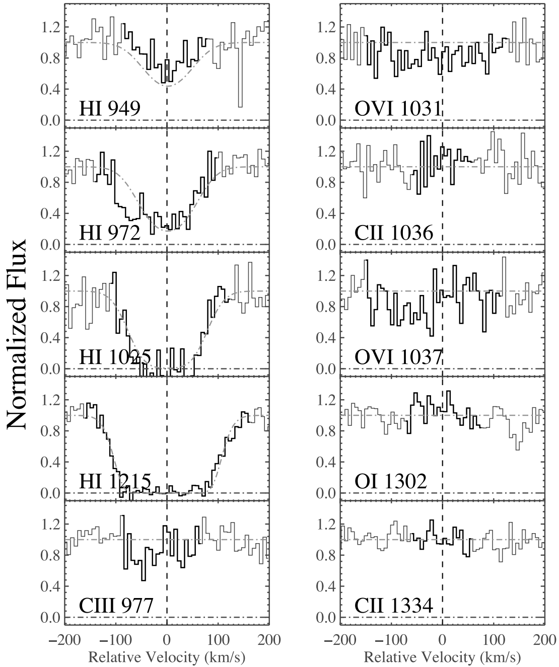
FIG. 14.—Velocity plot for z_{\text{abs}} = 0.14533 (see Fig. 1 description). \text{Ly}\delta is near the edge of the LiF 2A spectrum. C III is a >6\sigma detection (see Table 3). Both C II lines and O I are not detected at >3\sigma . The O VI doublet is not a confirmed detection; O VI \lambda 1037 is coincident with \text{Ly}\beta at z_{\text{abs}} = 0.15835 and is at the edge of LiF 1B and in a noisy region of STIS. The Voigt profile centroid is fixed at z_{\beta} = 0.14534 . (Note: the horizontal limits are from -200 to +200 km s ^{-1} .) [See the electronic edition of the Journal for a color version of this figure.]
