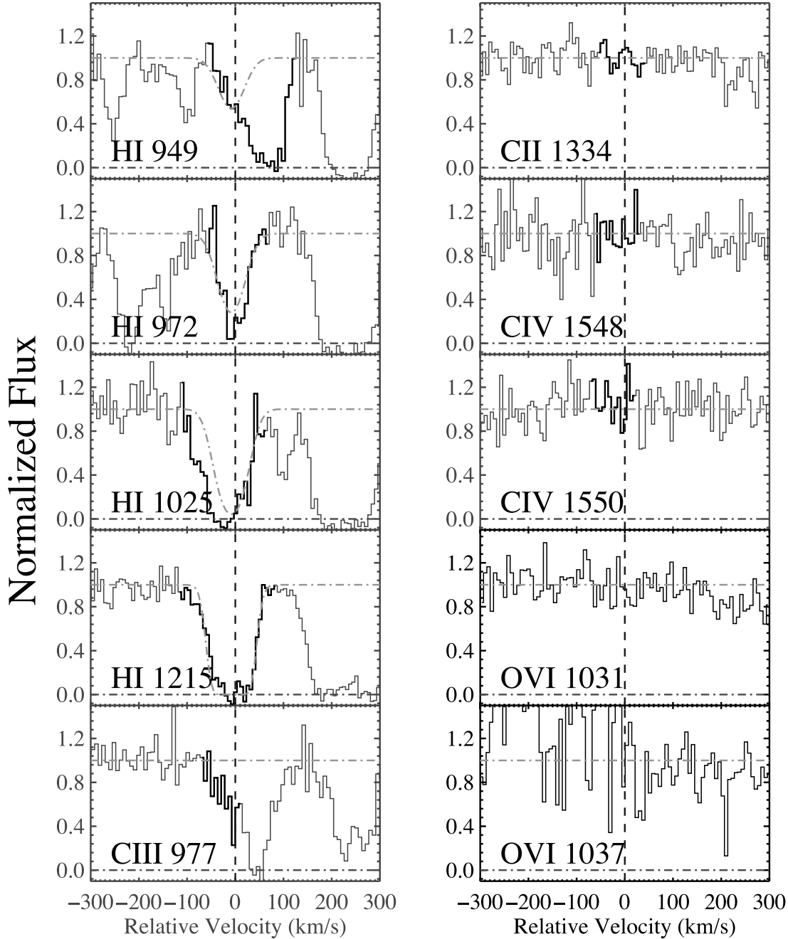
FIG. 7.—Velocity plot for z_{\text{abs}} = 0.09400 (see Fig. 1 description). Ly \beta , Ly \gamma , and Ly \delta are blended with Galactic Fe II \lambda 1121 , Galactic Fe II \lambda 1064 , and Galactic O I \lambda 1039 , respectively. C III is blended with Ly \beta at z_{\text{abs}} = 0.04222 . C II and the C IV doublet are not detected at 3\sigma . The region where the O VI doublet would be is shown. The Voigt profile centroid is fixed at z_{\gamma} = 0.09397 . [See the electronic edition of the Journal for a color version of this figure.]
