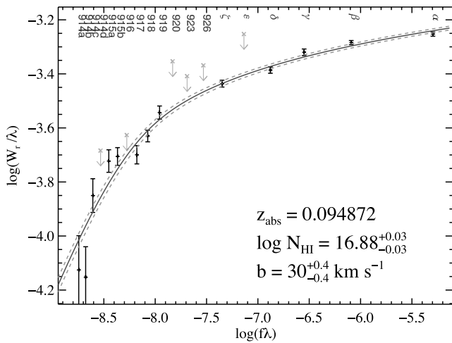
FIG. 11.— \text{H I} COG for z_{\text{abs}} = 0.09487 (see Fig. 2 description). This system is fitted well by a single-component COG model despite \text{Ly}\alpha having a multi-component line profile (see Fig. 9). [See the electronic edition of the Journal for a color version of this figure.]
