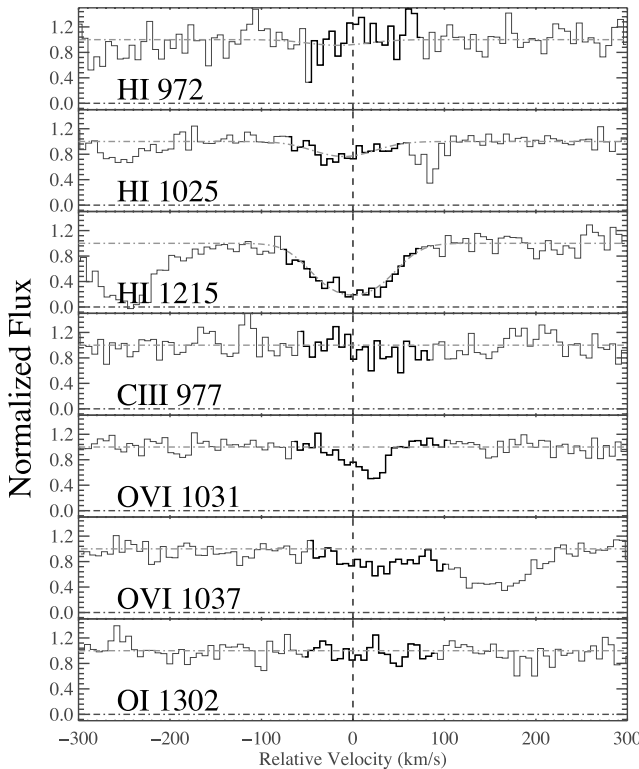
FIG. 18.—Velocity plot for z_{\text{abs}} = 0.22555 (see Fig. 1 description). O VI \lambda 1037 is slightly blended with Ly \alpha at z_{\text{abs}} = 0.04222 on the red side. Ly \gamma , C III, and O I are not detected at 3\sigma . The Voigt profile centroid is fixed at z_{\alpha} = 0.22555 . [See the electronic edition of the Journal for a color version of this figure.]
