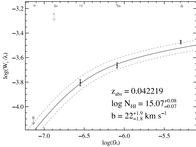
FIG. 4.—H I COG for z_{\text{abs}} = 0.04222 (see Fig. 2 description). Ly \epsilon , which is not detected at 3\sigma , is shown as a 2\sigma upper limit (square and arrow). Ly \delta is blended with Galactic N III. [See the electronic edition of the Journal for a color version of this figure.]
