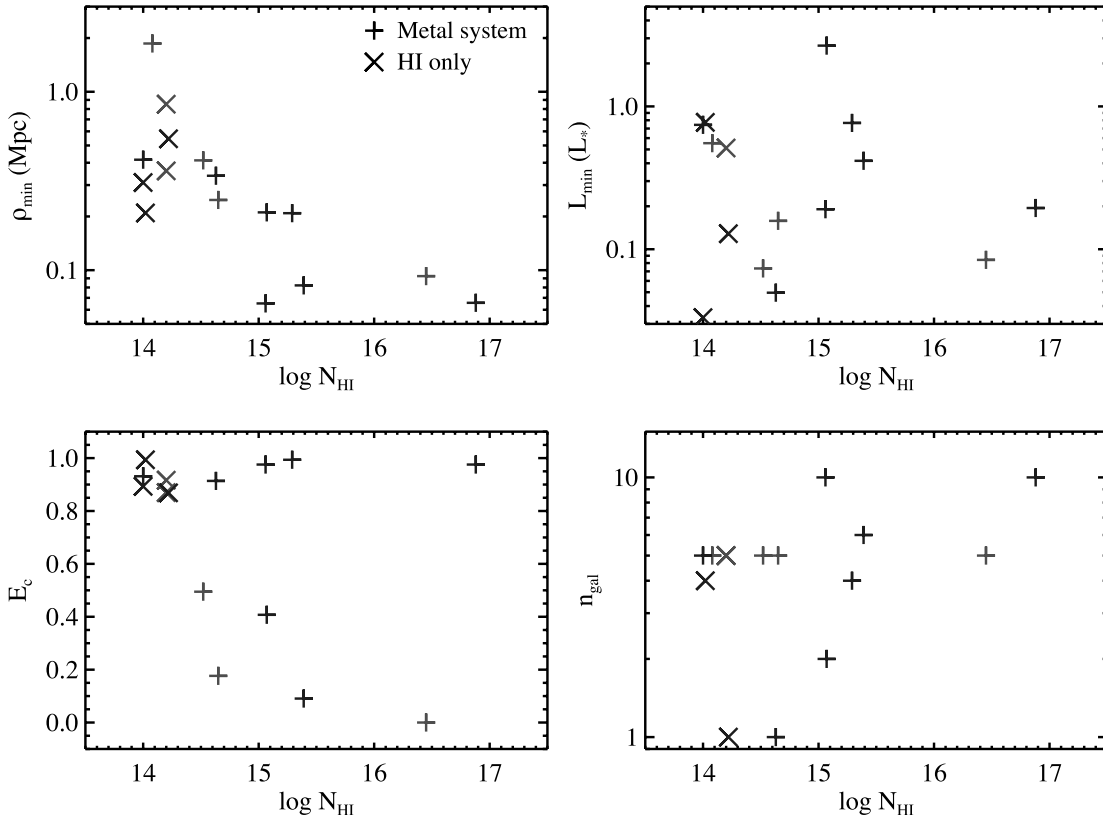
FIG. 24.—Impact parameter ( \rho_{\text{min}} ), luminosity ( L_{\text{min}} ), and spectral coefficient ( E_c ) of the closest galaxy with L > 0.1 L_* , \rho < 5 \text{ Mpc} , and |\delta v_{\text{gal}}| < 1000 \text{ km s}^{-1} for the absorbers with N_{\text{H I}} > 10^{14} \text{ cm}^{-2} at z_{\text{abs}} < 0.2 along the sight lines to PKS 0405–123 (lighter) and PKS 1302–102 (darker). The point types distinguish between metal-line systems (plus signs) and absorbers that only show \text{Ly}\alpha absorption (crosses). There appears to be a trend toward lower \rho_{\text{min}} values for higher N_{\text{H I}} value of the absorbers. (Note: in the current work, the absolute magnitude for L_* at z = 0 is 1 mag fainter than that used in Prochaska et al. 2006.) [See the electronic edition of the Journal for a color version of this figure.]
