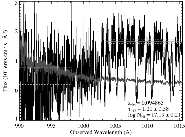
FIG. 10.—Lyman limit at z_{\text{abs}} = 0.09487 . We show our fits and conservative error estimates ( solid and dashed lines, respectively ) for the quasar continuum redward of the \lambda 912 break and the flux blueward. From the flux decrement, we measure the optical depth at the limit and the \text{H I} column density. The gray line is the error array of the spectrum. This portion of the spectrum is at the blue edge of LiF 1A, where the sensitivity decreases. [See the electronic edition of the Journal for a color version of this figure.]
