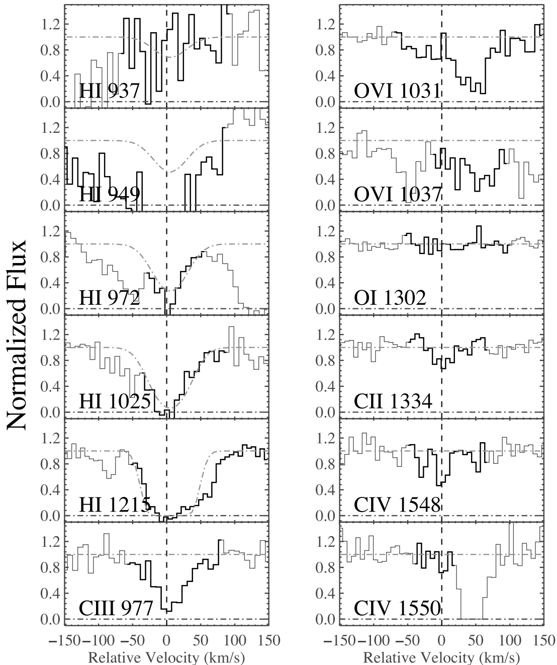
FIG. 3.—Velocity plot for z_{\text{abs}} = 0.04222 (see Fig. 1 description). The \text{Ly}\alpha profile shows two components on either side of v = 0 \text{ km s}^{-1} . C III is more aligned with the stronger, blueward component of \text{Ly}\alpha , while O VI is more aligned with the weaker, redward component. The Voigt profiles are based on a single-component COG model (see Fig. 4) with centroid fixed at z_{\gamma} = 0.04224 . O VI \lambda 1037 is blended with \text{H}_2 \lambda 1081.7 R(3) and is flanked by \text{H}_2 \lambda 1081.2 P(2) to the blue and Galactic F II \lambda 1081 to the red. \text{Ly}\beta , \text{Ly}\gamma , and \text{Ly}\delta are blended (see § 4.2). \text{Ly}\epsilon , O I, C II, and C IV \lambda 1550 are not detected at 3\sigma . The location of C IV \lambda 1550 spans an echelle order gap in STIS. [See the electronic edition of the Journal for a color version of this figure.]
