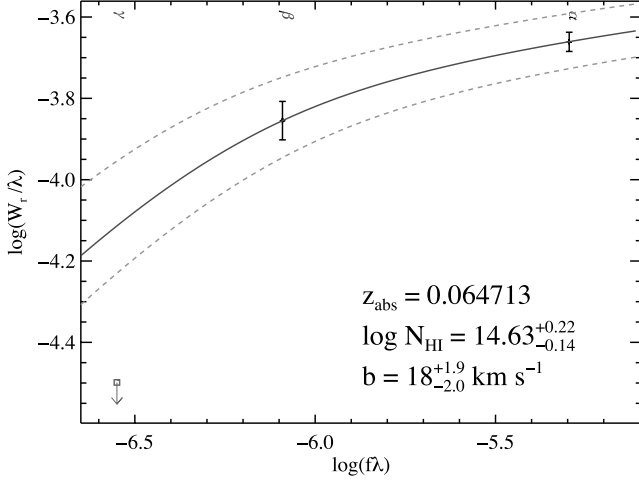
FIG. 6.—H I COG for z_{\text{abs}} = 0.06471 (see Fig. 2 description). Ly \gamma is not detected at 3\sigma but is consistent within 1\sigma with the single-component COG fit. This H I system is possibly multicomponent, as evidenced by the asymmetric Ly \alpha and Ly \beta profiles in Fig. 5. [See the electronic edition of the Journal for a color version of this figure.]
