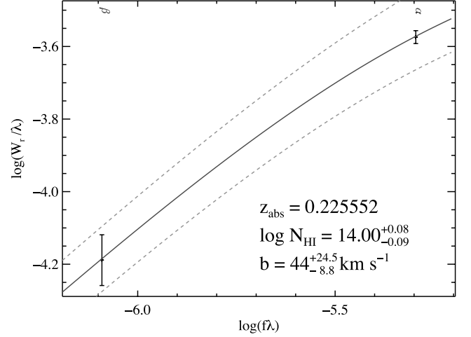
FIG. 19.—H I COG for z_{\text{abs}} = 0.22555 (see Fig. 2 description). [See the electronic edition of the Journal for a color version of this figure.]
