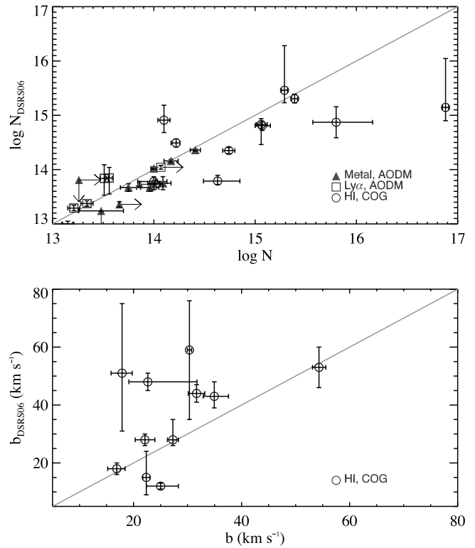
FIG. 21.—Comparison of column densities and Doppler parameters reported by D06 against those from our analysis. The categories denoted by symbol refer to the current work. The H I COG analysis \log N and b are circles; the AODM \log N are triangles for metal lines (i.e., C III and O VI) and squares for Ly \alpha . We generally agree with \log N_{\text{D06}} because the sum of potential components does not greatly affect the total column density (top). On the other hand, unresolved components tend to increase b_{\text{D06}} compared to our values, as discussed in D06 (bottom). [See the electronic edition of the Journal for a color version of this figure.]
