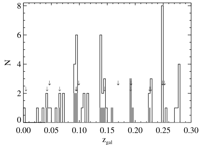
FIG. 22.—Histogram of 64 galaxies with z_{\text{gal}} \leq 0.3 in PKS 1302–102 field, binned to 1000 \text{ km s}^{-1} (open histogram). The filled histogram is galaxies within 5' , 95% complete to R \approx 19.5 . The arrows indicate the redshifts of the nine metal-line systems (lower) and the seven strong \text{Ly}\alpha absorbers (upper; see Table 7). There are groups of absorbers with |\delta v_{\text{abs}}| < 500 \text{ km s}^{-1} and with nearby galaxies that may be large-scale filaments at z_{\text{abs}} \approx 0.094 , 0.192 , and 0.225 . [See the electronic edition of the Journal for a color version of this figure.]
