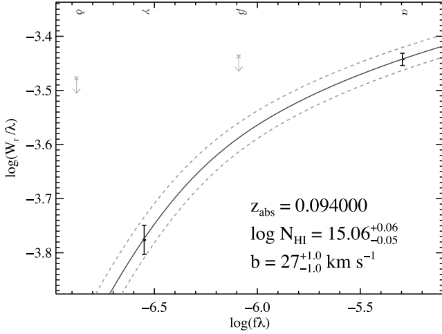
FIG. 8.—H I COG for z_{\text{abs}} = 0.09400 (see Fig. 2 description). The COG analysis only includes Ly \alpha and Ly \gamma because Ly \beta and Ly \delta were blended (see Fig. 7). Ly \gamma is blended with a weak Galactic line. Therefore, we conservatively consider the best fit to be an upper limit. [See the electronic edition of the Journal for a color version of this figure.]
